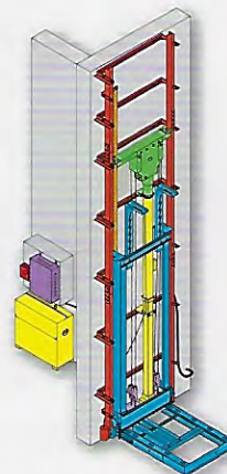
Excelelevator Roped Hydraulic Series 114 Capacity 1,000 lbs
